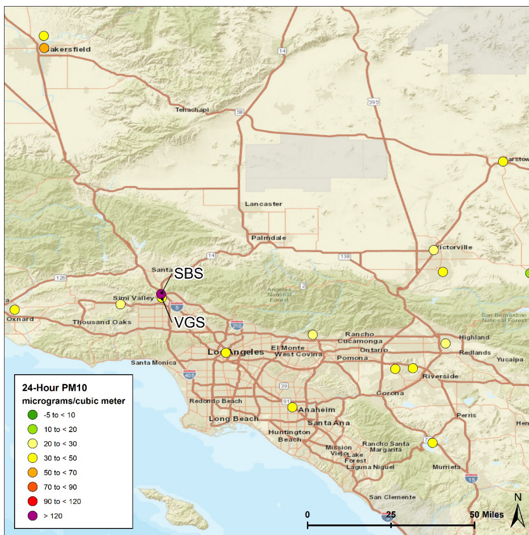
Figure 3-4. PM 10 concentrations at sites across the Los Angeles area on October 30, 2023. Colors correspond to 24-hr PM 10 concentrations in µg/m 3 . Note: no sites besides the Landfill site (labeled as SBS) within the map domain recorded 24-hr PM 10 concentrations above the federal standard. No active wildfire events were within the map domain on this day.
