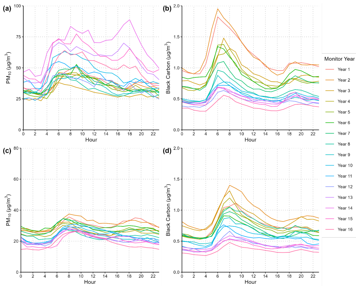
Figure B-1. Mean PM 10 and BC concentrations by hour for the 16 monitoring years at the Landfill (a, b) and Community (c, d) sites.
