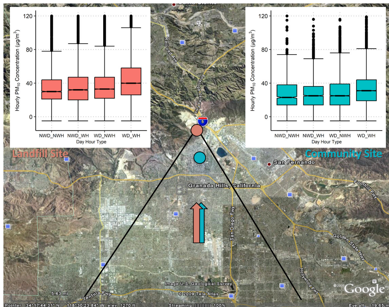
Figure 5-8. Notched box whisker plots of 16-yr hourly PM 10 concentrations for southerly (“From SoCAB”) wind sectors (as displayed in Figure 5-4) for working days (WD), non-working days (NWD), working hours (WH), and non-working hours (NWH) within those days for the Landfill (red) and Community (blue) monitor sites. Outliers over 120 µg/m 3 are not displayed.
