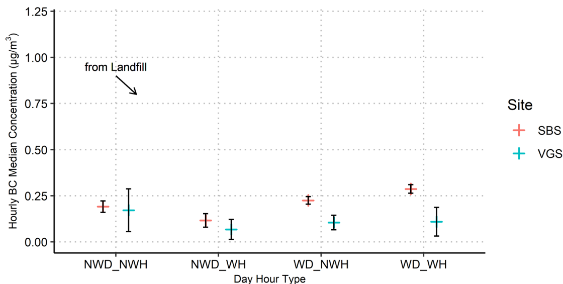
Figure 5-22. Year 16 (2023) hourly median BC concentrations for northerly ("From Landfill") wind sectors (as displayed in Figure 5-4) for working days (WD), non-working days (NWD), working hours (WH), and non-working hours (NWH) within those days for the Landfill (red) and Community (blue) monitor sites. 95% confidence intervals are shown in black.
