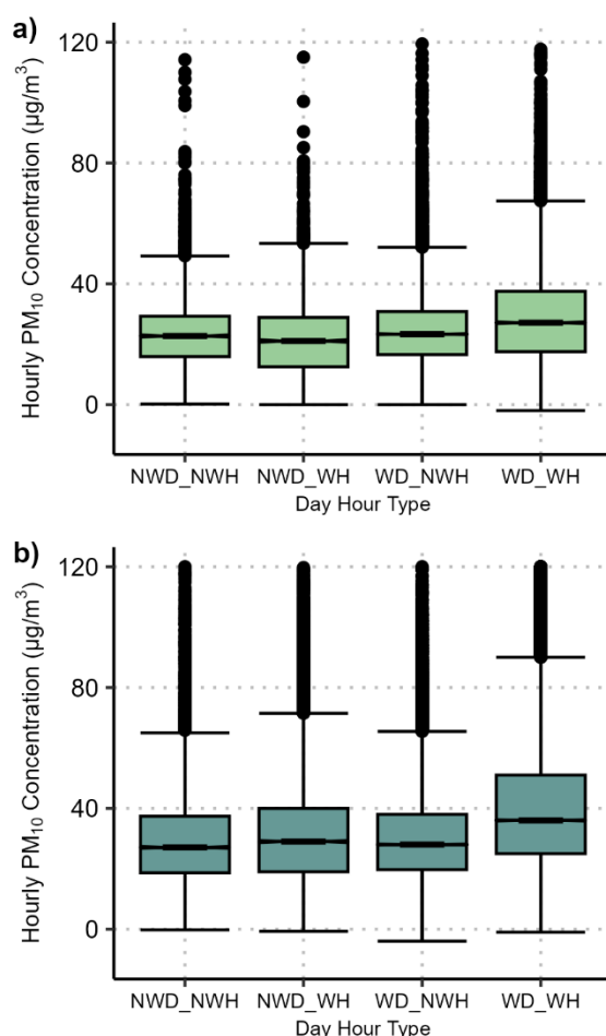
Figure 5-15. Hourly PM 10 median concentrations for (a) Burbank (2008-2014) and (b) Los Angeles (2008-2023) for working days (WD), non-working days (NWD), working hours (WH), and non-working hours (NWH).
