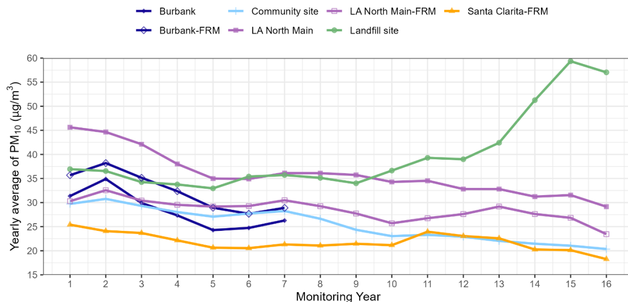
Figure 4-2. Rolling 3-yr annual average PM 10 concentrations for the Landfill and Community sites, and three regional monitoring sites for Monitoring Year 1–Year 16 (e.g., Monitoring Year 1 refers to Nov. 22, 2007–Nov. 21, 2008). Additional FRM data collected at the Los Angeles site and at the Burbank site are also included.
