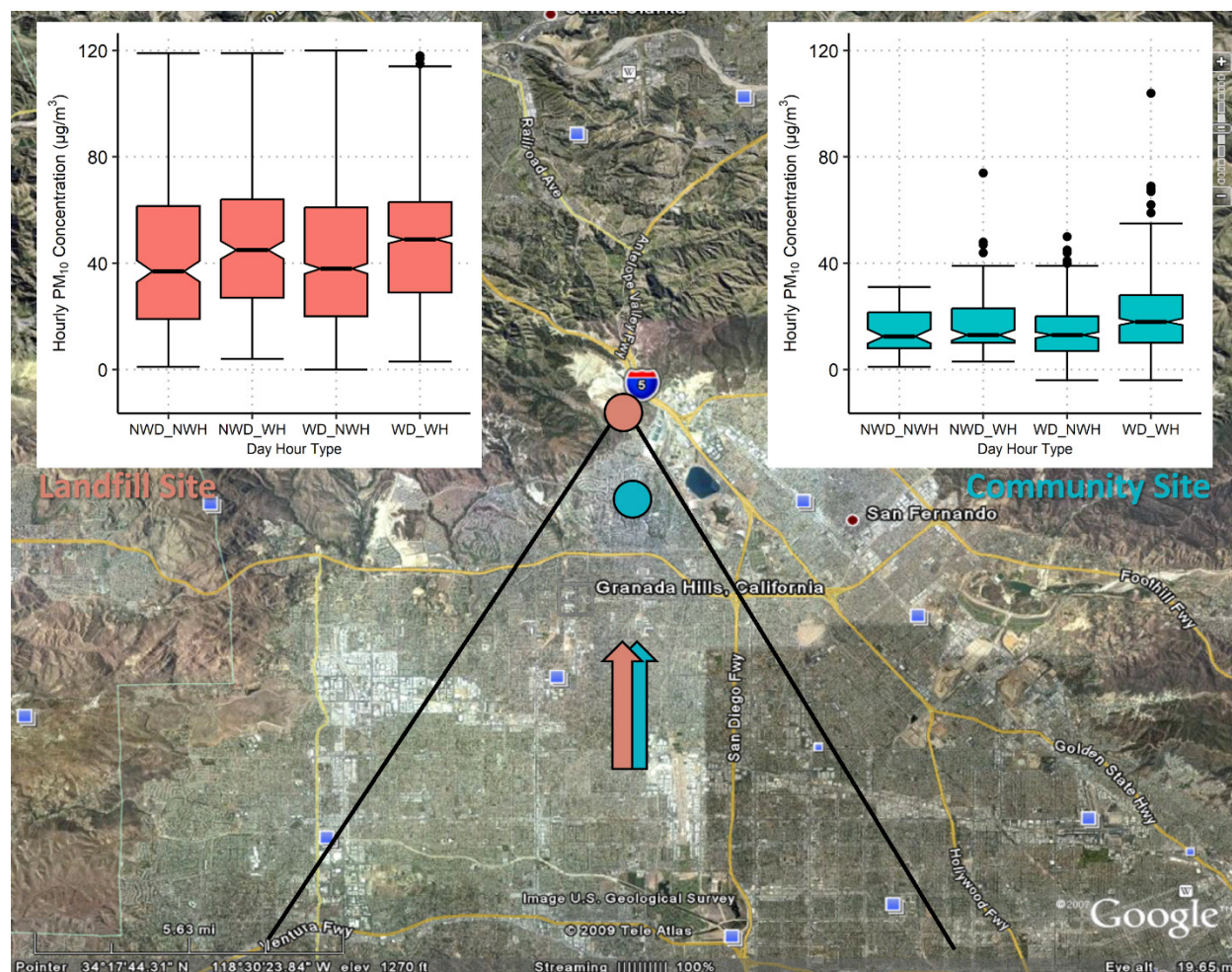
Figure 5-10. Notched box whisker plots of Year 16 (2023) hourly PM 10 concentrations for southerly (“From SoCAB”) wind sectors (as displayed in Figure 5-4) for working days (WD), non-working days (NWD), working hours (WH), and non-working hours (NWH) within those days for the Landfill (red) and Community (blue) monitor sites. Outliers over 120 µg/m 3 are not displayed.
