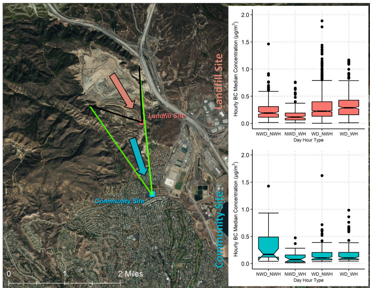
Figure 5-18. Notched box whisker plots of Year 16 (2023) hourly average BC concentrations for northerly (“From Landfill”) wind sectors (as displayed in Figure 5-4) for working days (WD), non-working days (NWD), working hours (WH), and non-working hours (NWH) within those days for the Landfill (red) and Community (blue) monitor sites. Outliers over 2 \mu\text{g}/\text{m}^3 are not displayed.
