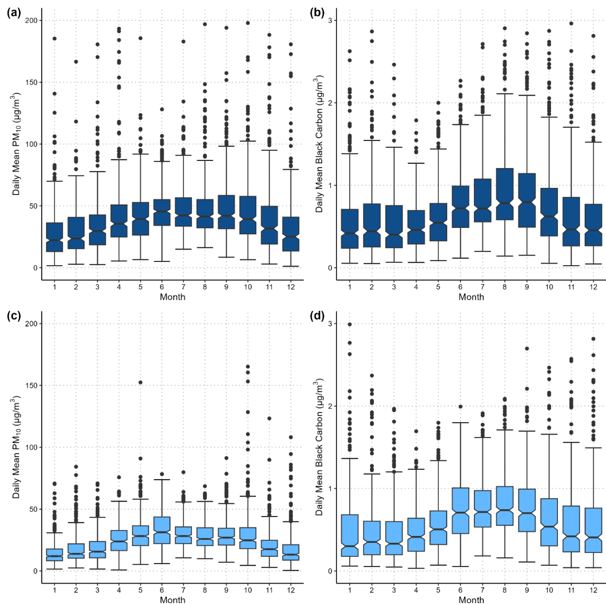
Figure B-2. Distribution of daily mean PM 10 and BC concentrations by month across all 15 monitor years (2007–2023) at the Landfill (a, b) and Community (c, d) sites. Note: BC outliers greater than 3 µg/m 3 and PM 10 outliers greater than 200 µg/m 3 are excluded.
