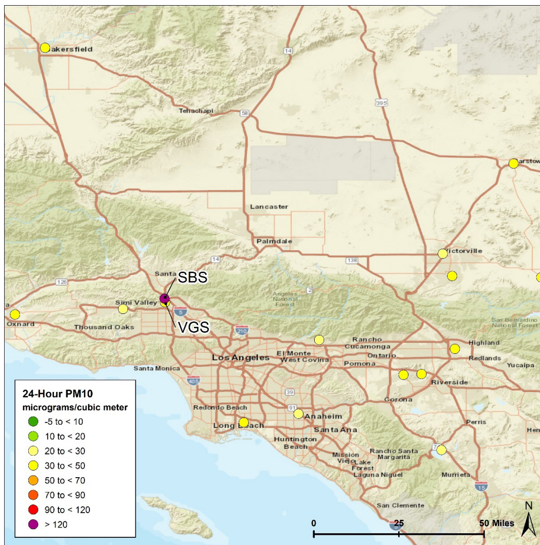
Figure 3-2. PM 10 concentrations at sites across the Los Angeles area on April 19, 2023. Colors correspond to 24-hr PM 10 concentrations in µg/m 3 . Note: no sites besides the Landfill site (labeled as SBS) within the map domain recorded 24-hr PM 10 concentrations above the federal standard. No active wildfire events were within the map domain on this day.
