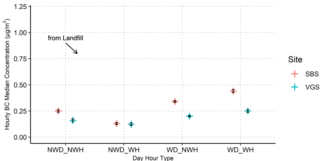
Figure 5-20. Sixteen-yr hourly median BC concentrations for northerly ("From Landfill") wind sectors (as displayed in Figure 5-4) for working days (WD), non-working days (NWD), working hours (WH), and non-working hours (NWH) within those days for the Landfill (red) and Community (blue) monitor sites. 95% confidence intervals are shown in black.
