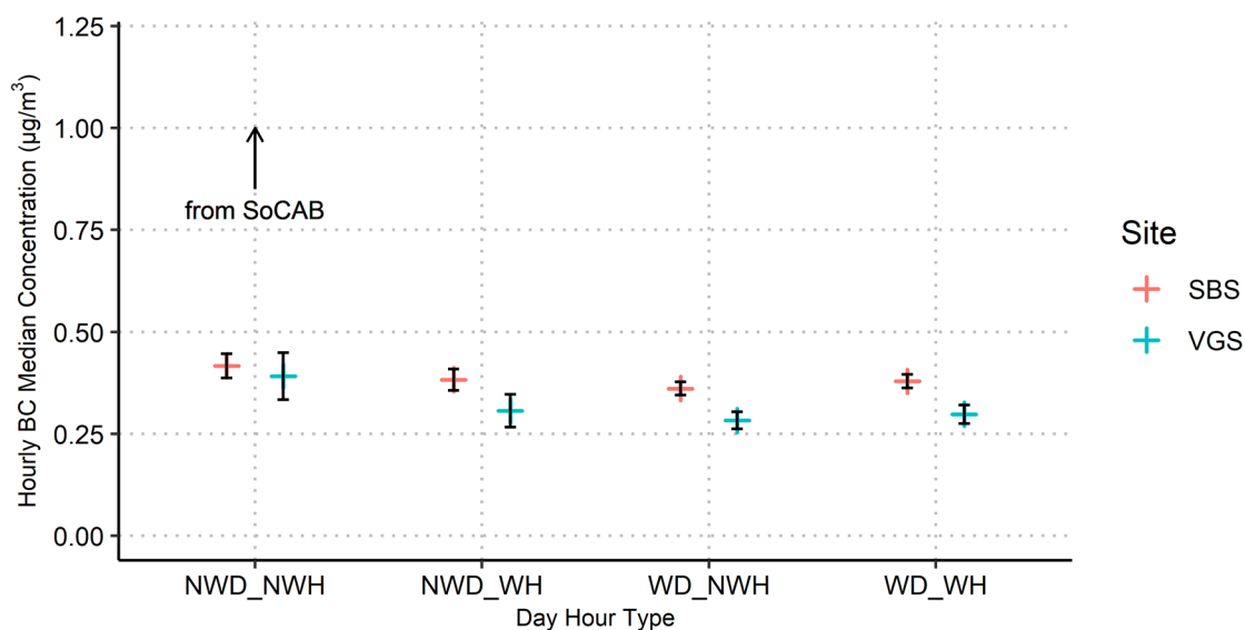
Figure 5-23. Year 16 (2023) hourly median BC concentrations for northerly ("From SoCAB") wind sectors (as displayed in Figure 5-4) for working days (WD), non-working days (NWD), working hours (WH), and non-working hours (NWH) within those days for the Landfill (red) and Community (blue) monitor sites. 95% confidence intervals are shown in black.
