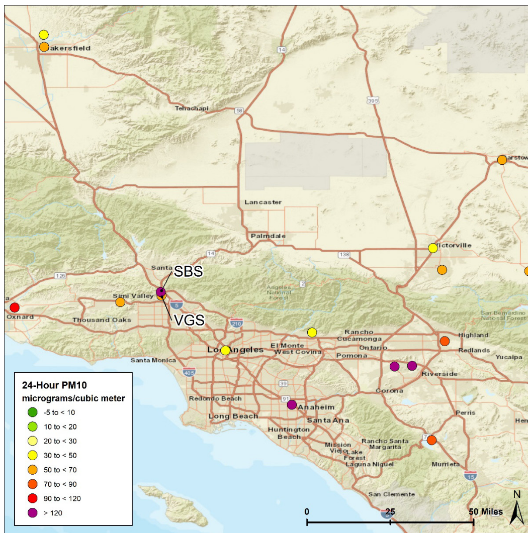
Figure 3-3. PM 10 concentrations at sites across the Los Angeles area on October 29, 2023. Colors correspond to 24-hr PM 10 concentrations in \mu\text{g}/\text{m}^3 . Note: one other site (within the left map domain) recorded 24-hr PM 10 concentrations above the federal standard. No active wildfire events were within the map domain on this day.
