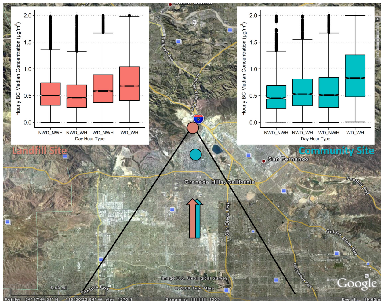
Figure 5-17. Notched box whisker plots of 16-yr hourly average BC concentrations for southerly (“From SoCAB”) wind sectors (as displayed in Figure 5-4) for working days (WD), non-working days (NWD), working hours (WH), and non-working hours (NWH) within those days for the Landfill (red) and Community (blue) monitor sites. Outliers over 2 \mu\text{g}/\text{m}^3 are not displayed.
