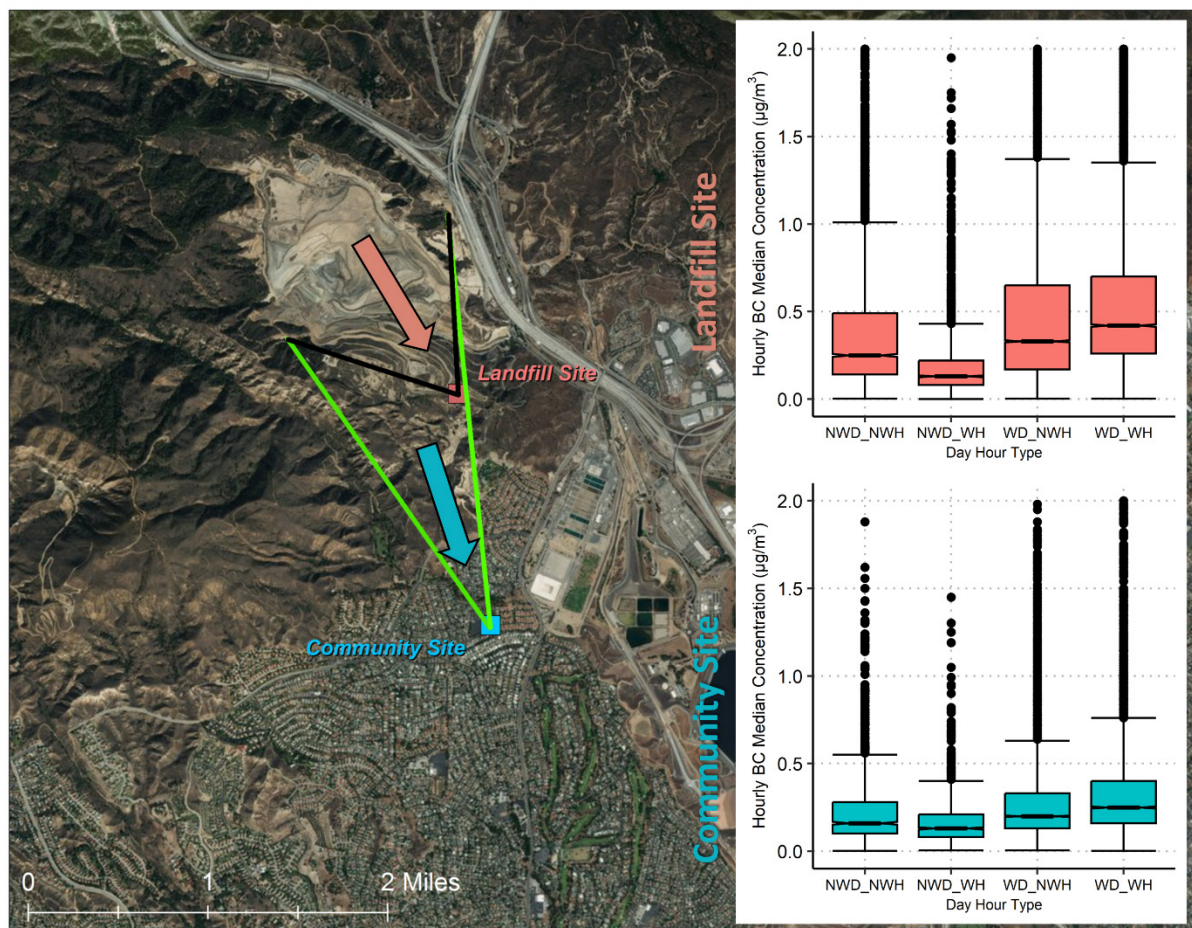
Figure 5-16. Notched box whisker plots of 16-yr hourly average BC concentrations for northerly (“From Landfill”) wind sectors (as displayed in Figure 5-4) for working days (WD), non-working days (NWD), working hours (WH), and non-working hours (NWH) within those days for the Landfill (red) and Community (blue) monitor sites. Outliers over 2 \mu\text{g}/\text{m}^3 are not displayed.
