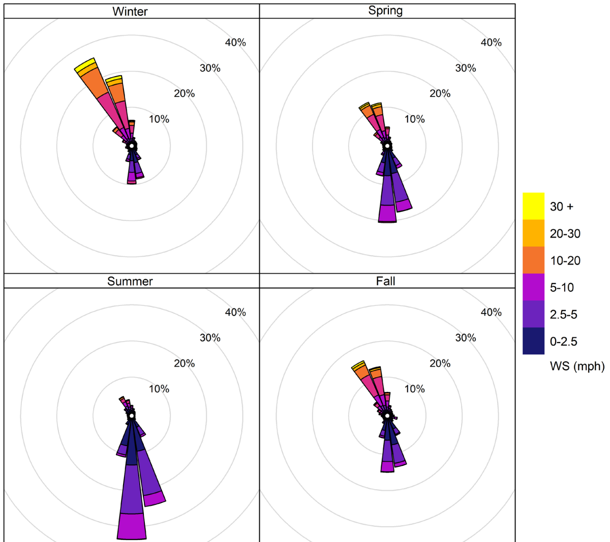
Figure B-4. Seasonal wind roses based on hourly data collected at the Landfill site from 2007-2023.
