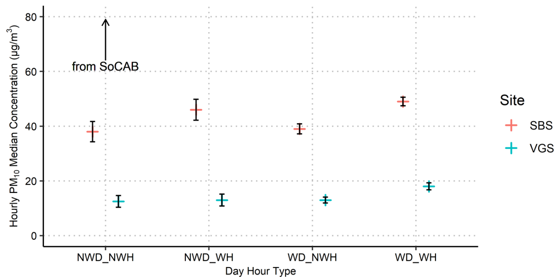
Figure 5-14. Year 16 (2023) hourly PM 10 median concentrations for northerly ("From SoCAB") wind sectors (as displayed in Figure 5-4) for working days (WD), non-working days (NWD), working hours (WH), and non-working hours (NWH) within those days for the Landfill (red) and Community (blue) monitor sites. 95% confidence intervals are shown in black.
