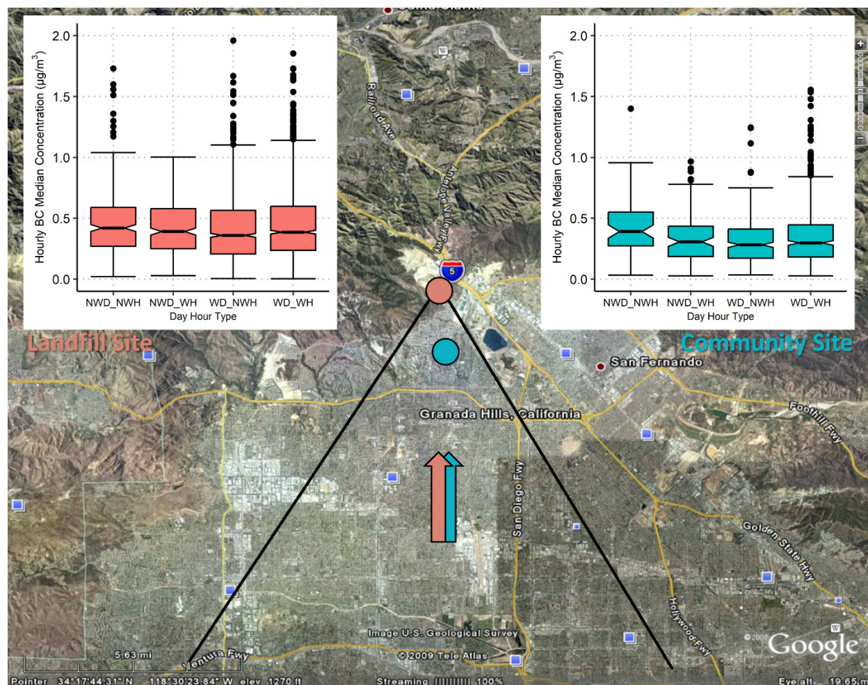
Figure 5-19. Notched box whisker plots of Year 16 (2023) hourly average BC concentrations for southerly ("From SoCAB") wind sectors (as displayed in Figure 5-4) for working days (WD), non-working days (NWD), working hours (WH), and non-working hours (NWH) within those days for the Landfill (red) and Community (blue) monitor sites. Outliers over 2 µg/m 3 are not displayed.
