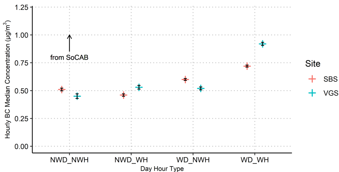
Figure 5-21. Sixteen-yr hourly median BC concentrations for northerly ("From SOCAB") wind sectors (as displayed in Figure 5-4) for working days (WD), non-working days (NWD), working hours (WH), and non-working hours (NWH) within those days for the Landfill (red) and Community (blue) monitor sites. 95% confidence intervals are shown in black.
