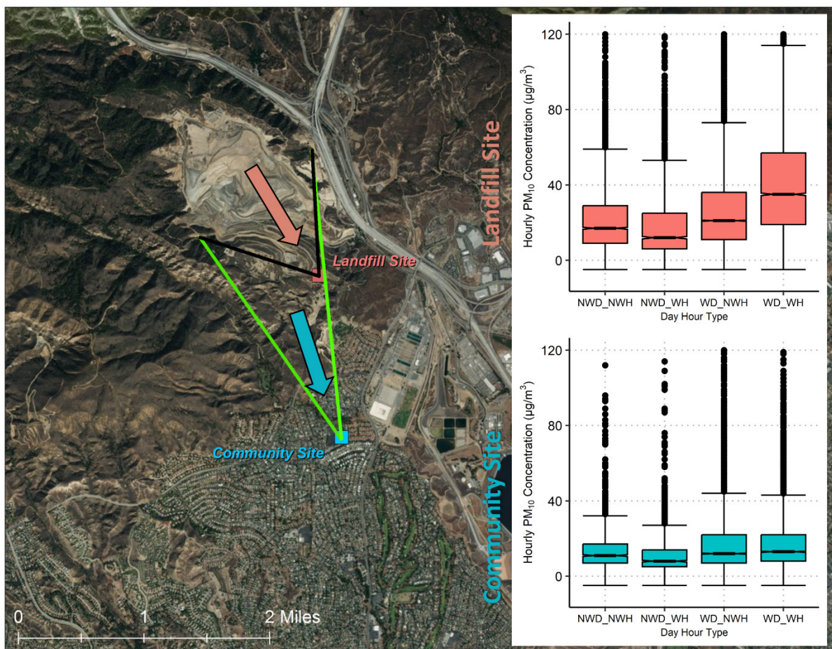
Figure 5-7. Notched box whisker plots of 16-yr hourly PM 10 concentrations for northerly ("From Landfill") wind sectors (as displayed in Figure 5-4) for working days (WD), non-working days (NWD), working hours (WH), and non-working hours (NWH) within those days for the Landfill (red) and Community (blue) monitor sites. Outliers over 120 µg/m 3 are not displayed.
