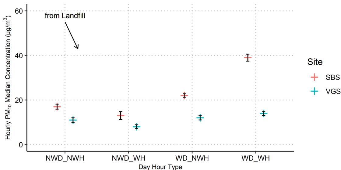
Figure 5-11. Sixteen-yr hourly PM 10 median concentrations for northerly (“From Landfill”) wind sectors (as displayed in Figure 5-4) for working days (WD), non-working days (NWD), working hours (WH), and non-working hours (NWH) within those days for the Landfill (red) and Community (blue) monitor sites. 95% confidence intervals are shown in black.
