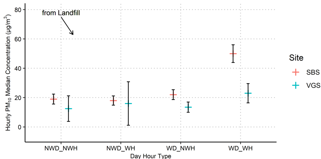
Figure 5-13. Year 16 (2023) hourly PM 10 median concentrations for northerly ("From Landfill") wind sectors (as displayed in Figure 5-4) for working days (WD), non-working days (NWD), working hours (WH), and non-working hours (NWH) within those days for the Landfill (red) and Community (blue) monitor sites. 95% confidence intervals are shown in black. Note that confidence intervals are a function of the number of data points; fewer data points lead to a wider interval and less certainty about where the median falls.
