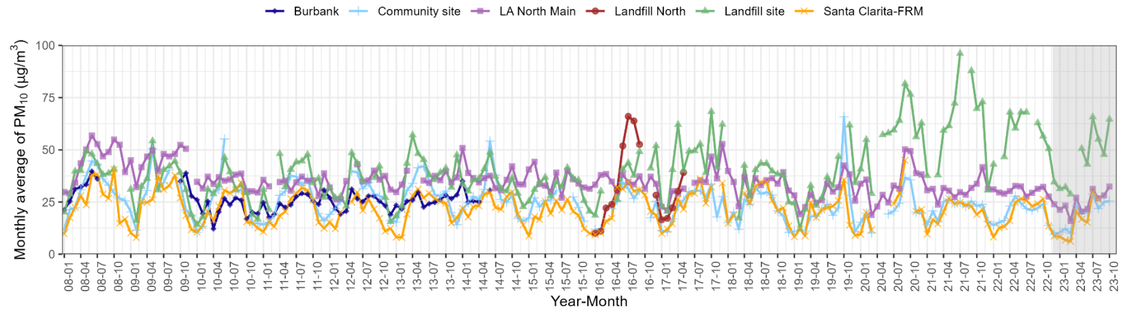
Figure 4-1. Monthly average PM 10 concentrations for the Landfill, Landfill North (in operation from June 2016 until May 2017), and Community sites, and three regional monitoring sites for 2008–2023. The Santa Clarita site reports integrated 24-hr samples of filters on a one-in-six-day schedule. As of June 30, 2014, the Burbank site is no longer actively reporting PM 10 data. The current year (Year 16) time period is shaded in grey.
