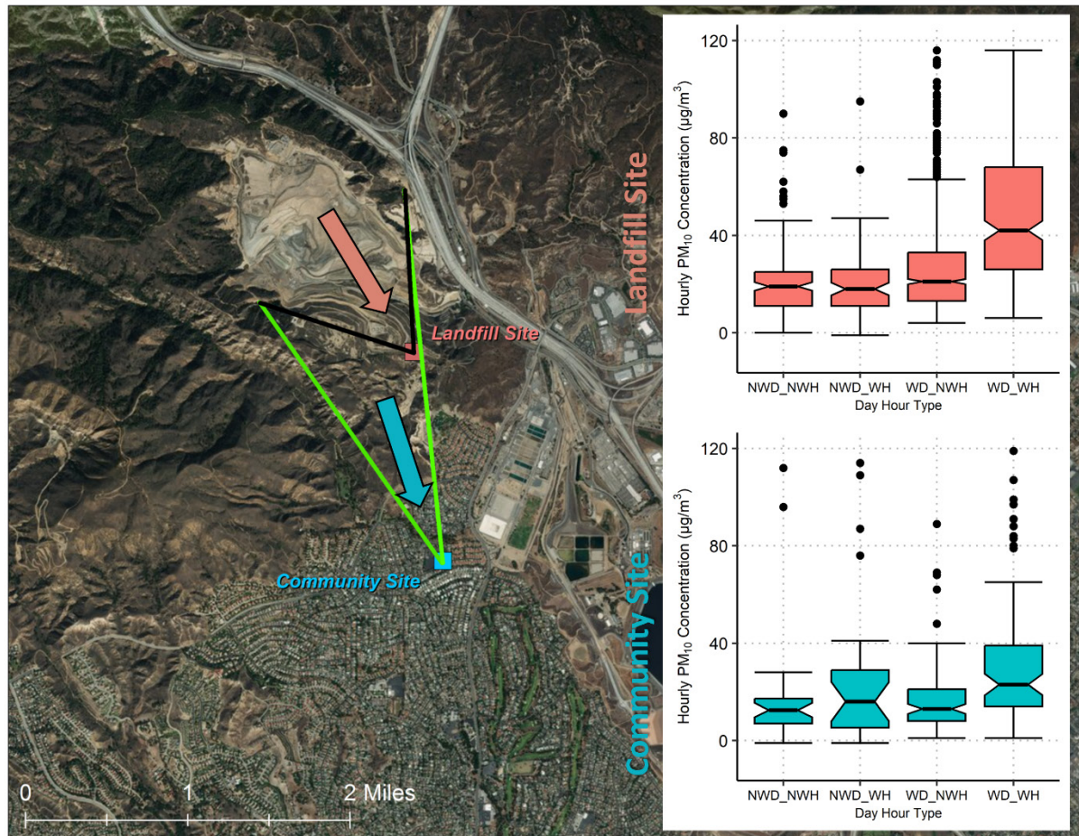
Figure 5-9. Notched box whisker plots of Year 16 (2023) hourly PM 10 concentrations for northerly (“From Landfill”) wind sectors (as displayed in Figure 5-4) for working days (WD), non-working days (NWD), working hours (WH), and non-working hours (NWH) within those days for the Landfill (red) and Community (blue) monitor sites. Outliers over 120 µg/m 3 are not displayed.
