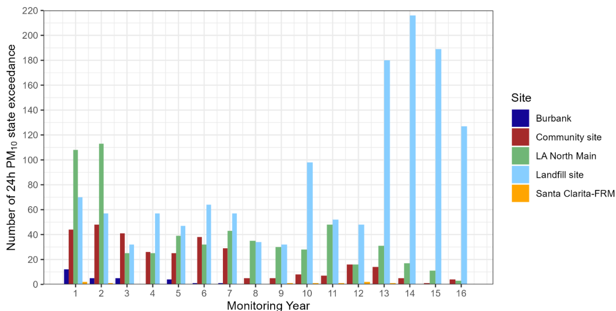
Figure 3-6. Number of state exceedances of 24-hr PM 10 at the Landfill, Community, and regional monitoring sites by year over the 16-yr study period. (e.g., Monitoring Year 1 refers to Nov. 22, 2007–Nov. 21, 2008).
