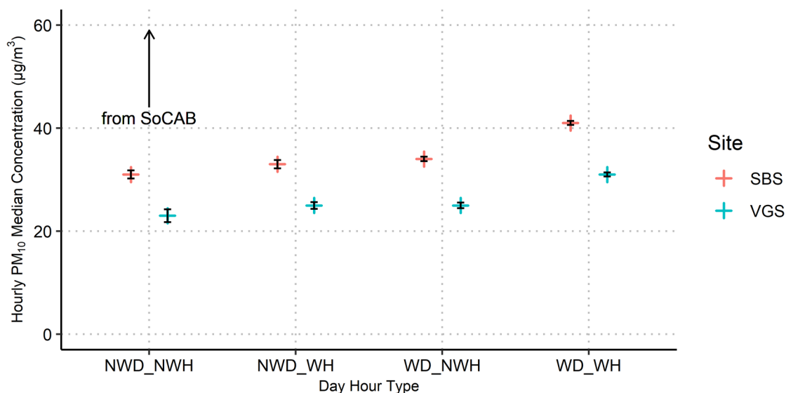
Figure 5-12. Sixteen-yr hourly PM 10 median concentrations for northerly (“From SoCAB”) wind sectors (as displayed in Figure 5-4) for working days (WD), non-working days (NWD), working hours (WH), and non-working hours (NWH) within those days for the Landfill (red) and Community (blue) monitor sites. 95% confidence intervals are shown in black.
