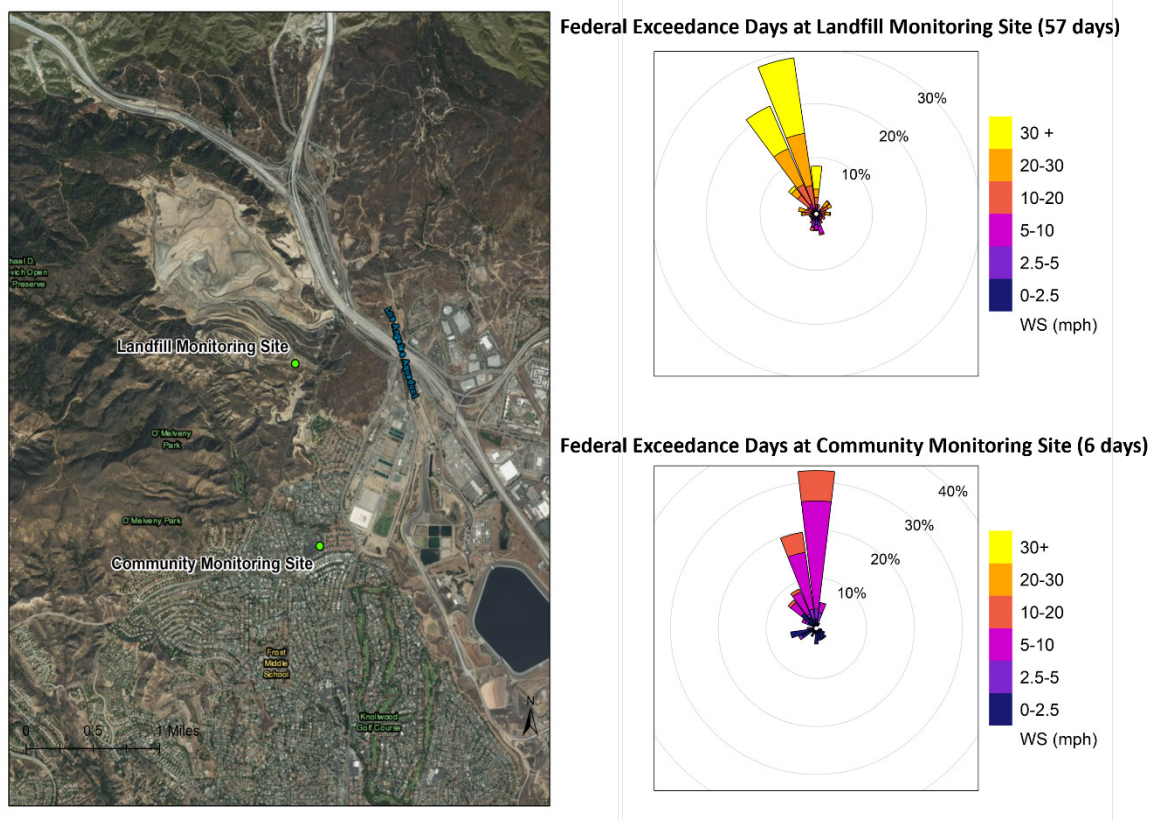
Figure 3-5. Wind rose from federal exceedance days during 16 continuous monitoring years at the Landfill (top right) and Community (bottom right) sites. Wind data at the Community site are replaced with those from the Reseda site since Year 11.
