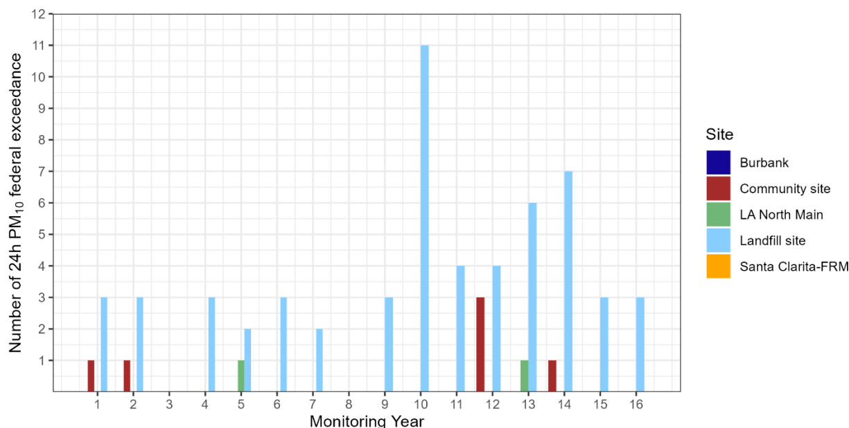
Figure 3-1. The number of federal exceedances of 24-hr PM 10 at the Landfill, Community, and regional monitoring sites by year over the 16-yr study period. (e.g., Monitoring Year 1 refers to Nov. 22, 2007-Nov. 21, 2008).
