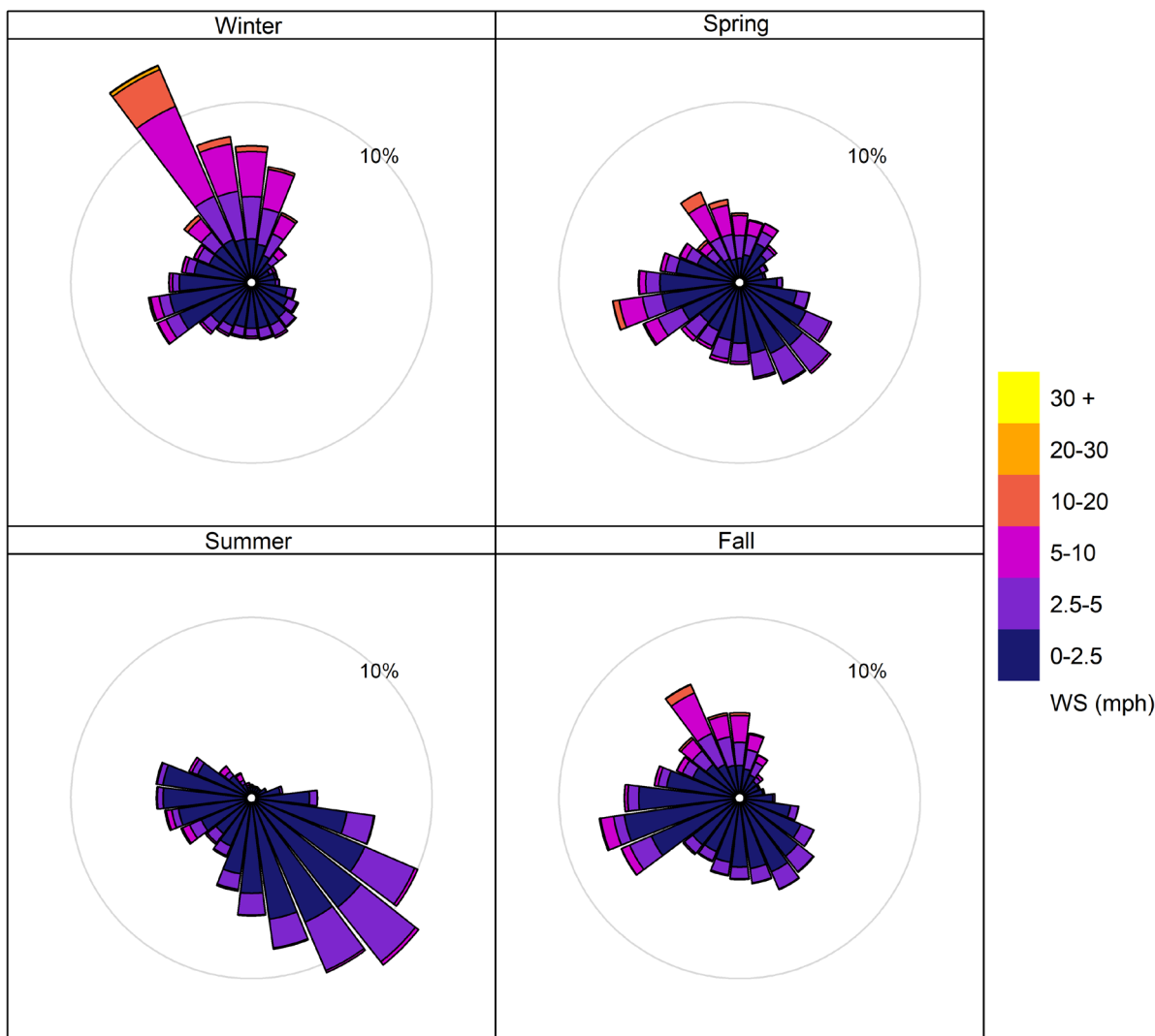
Figure B-5. Seasonal wind roses based on hourly data collected at the Community site from 2007-2023. Data since the 11th report year are replaced with wind data from the Reseda site.
